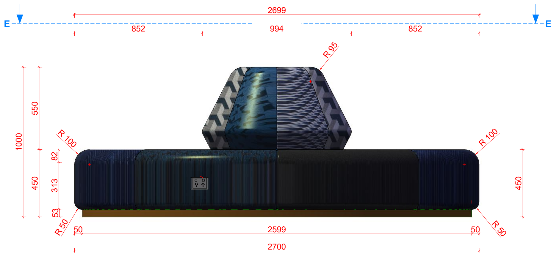
08 ELEVATION Scale@NTC
