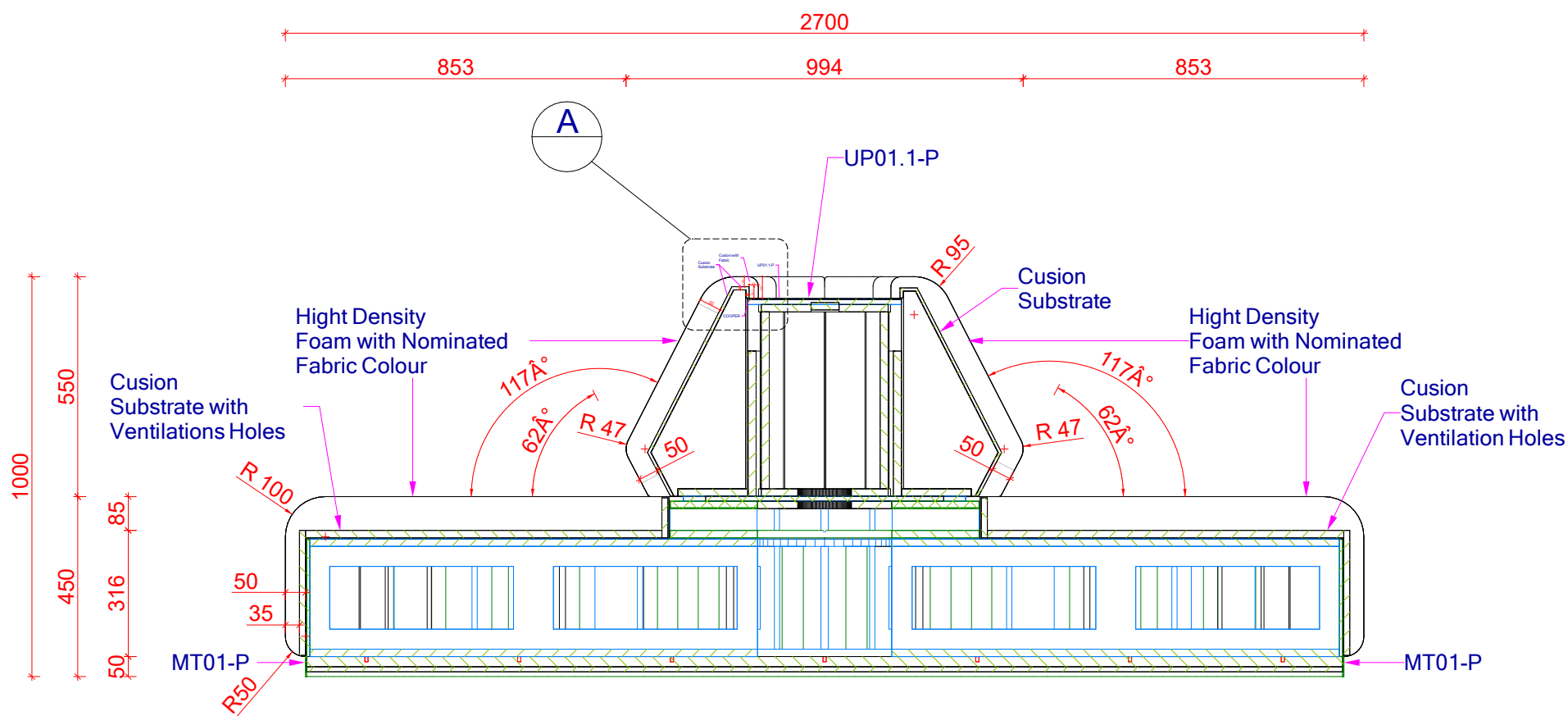
08 ELEVATION Scale@NTC
