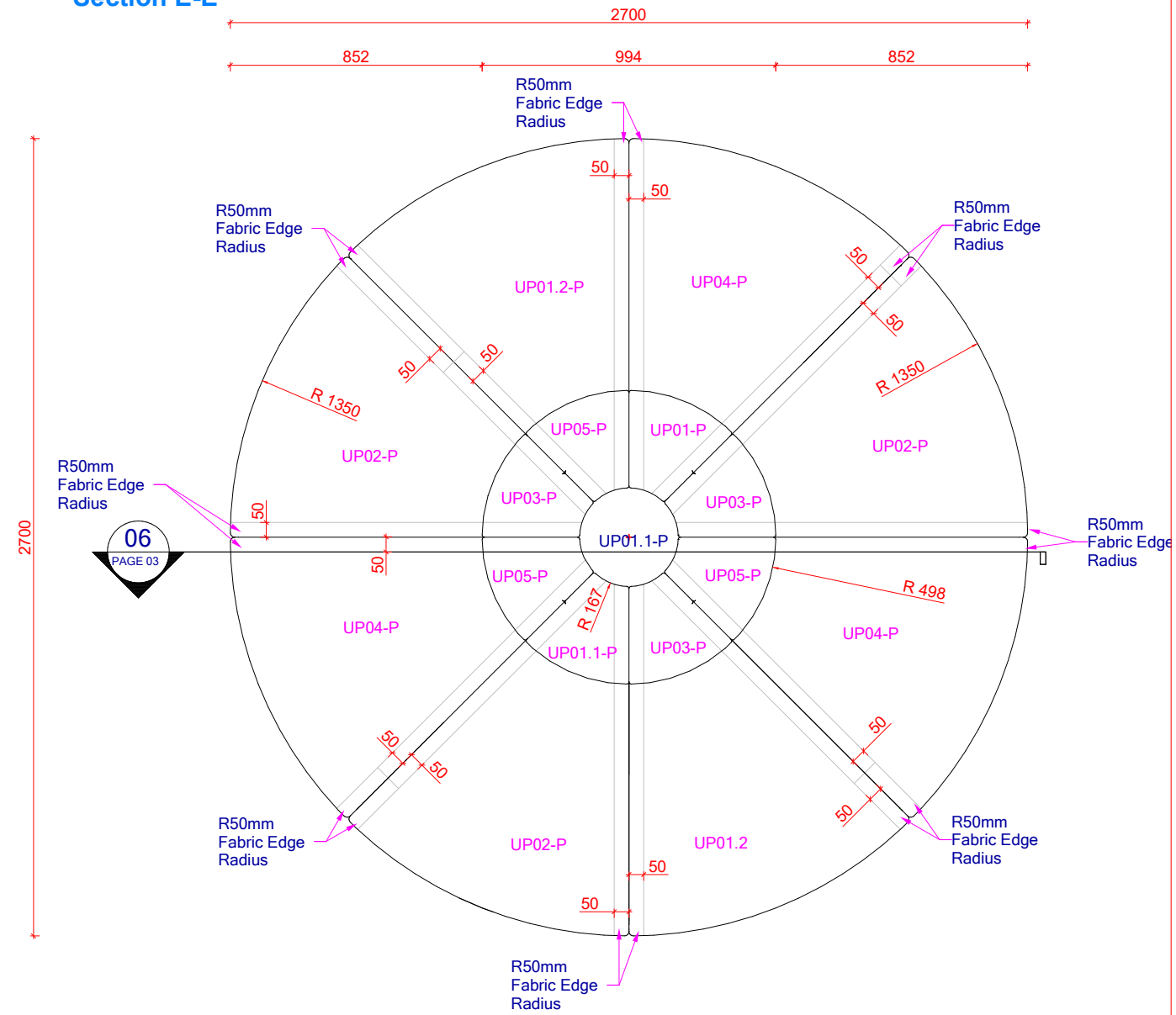
Section E-E
