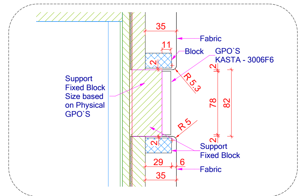
B POWER POINT DETAIL Scale@NTC
